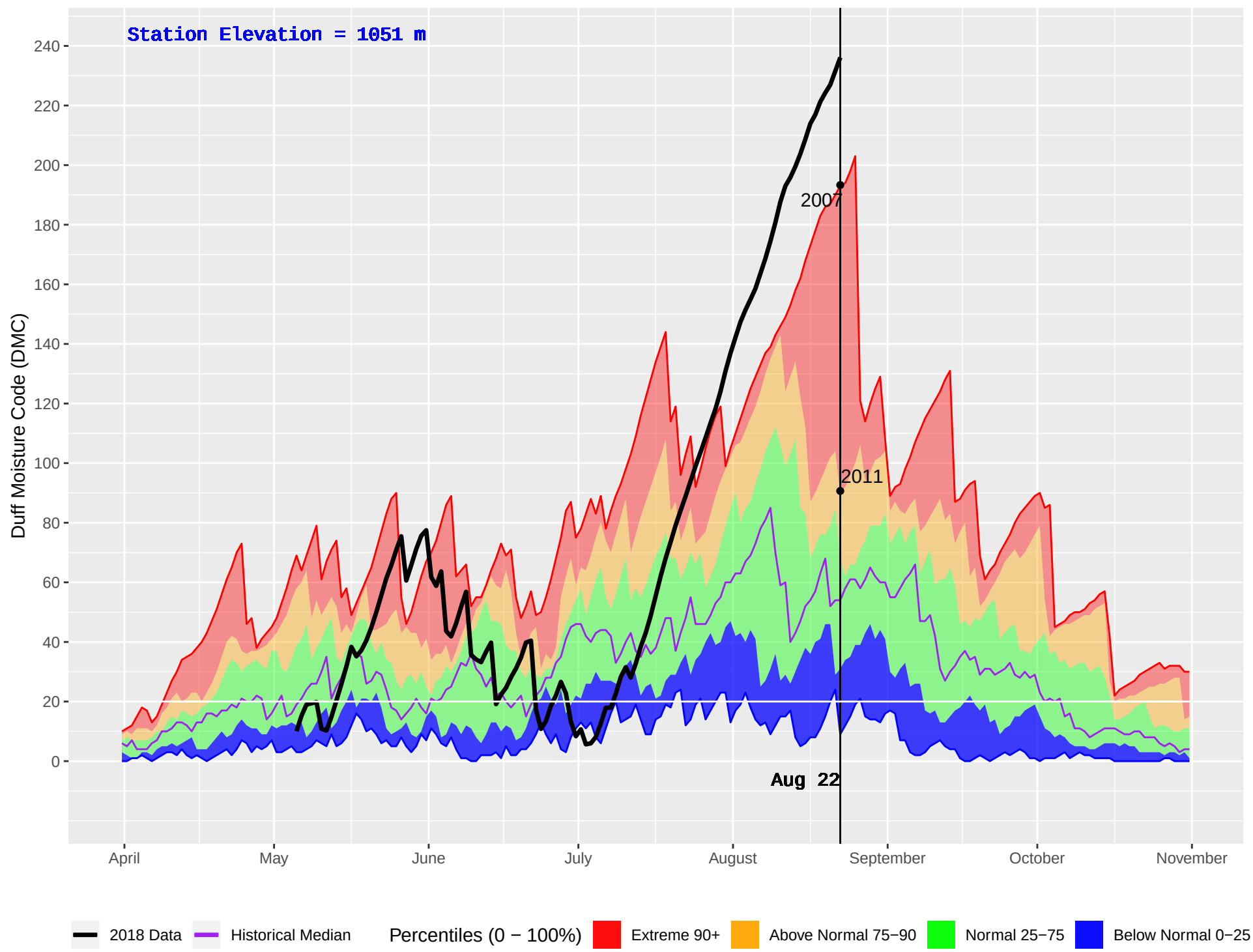
GOATHAVEN (886) : Historical (2005–2016) and Current (2018) Daily Duff Moisture Code (DMC)
