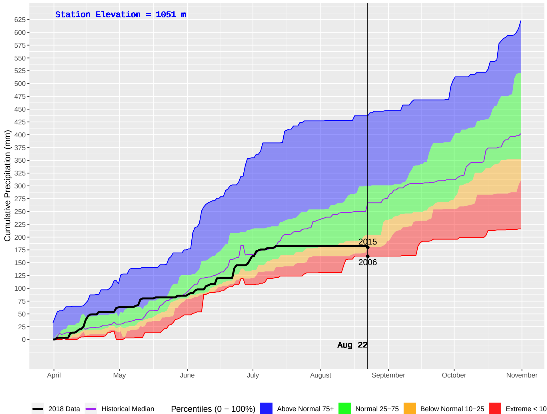
GOATHAVEN (886) : Historical (2005–2016) and Current (2018) Daily Cumulative Precipitation
