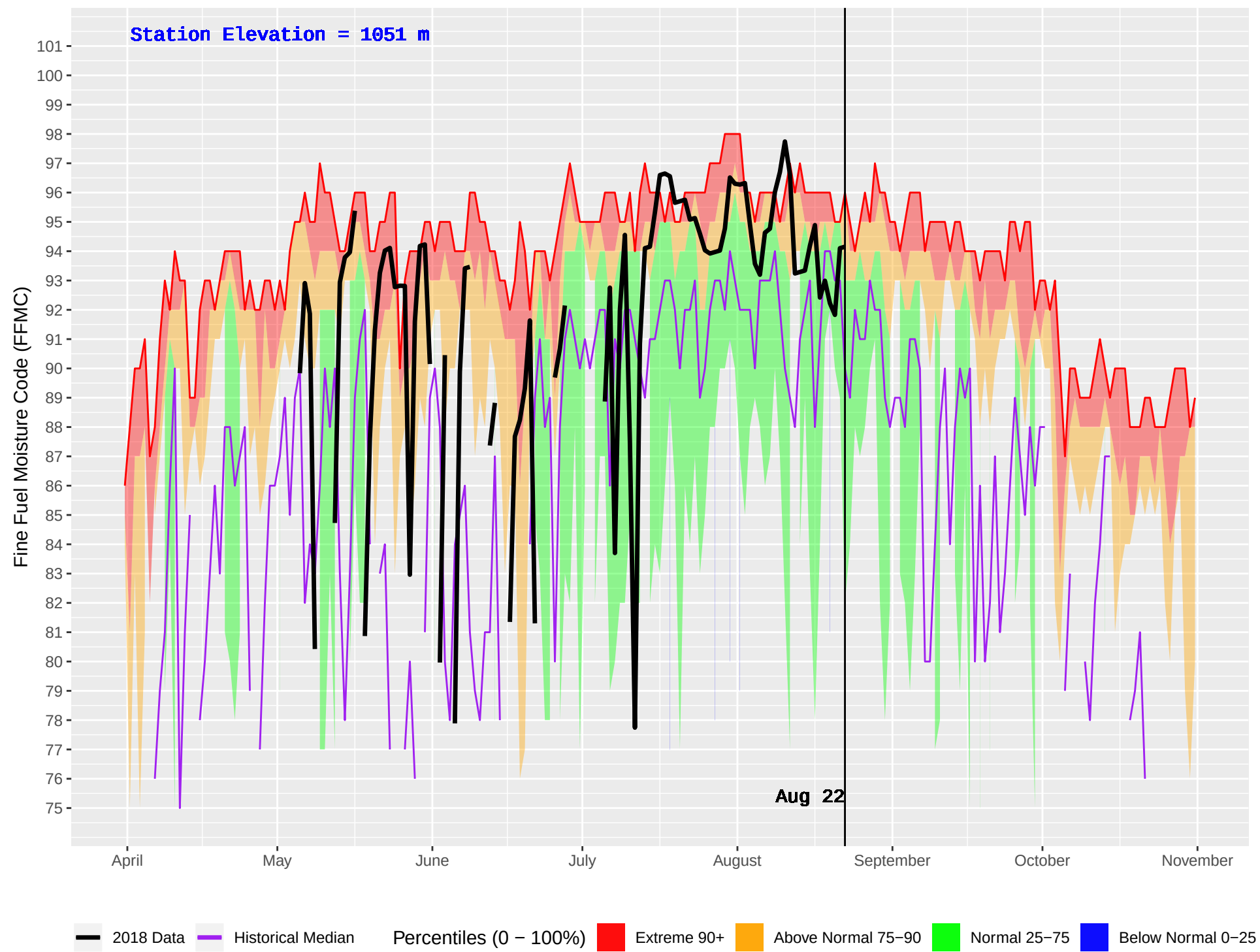
GOATHAVEN (886) : Historical (2005–2016) and Current (2018) Daily Fine Fuel Moisture Code (FFMC)
