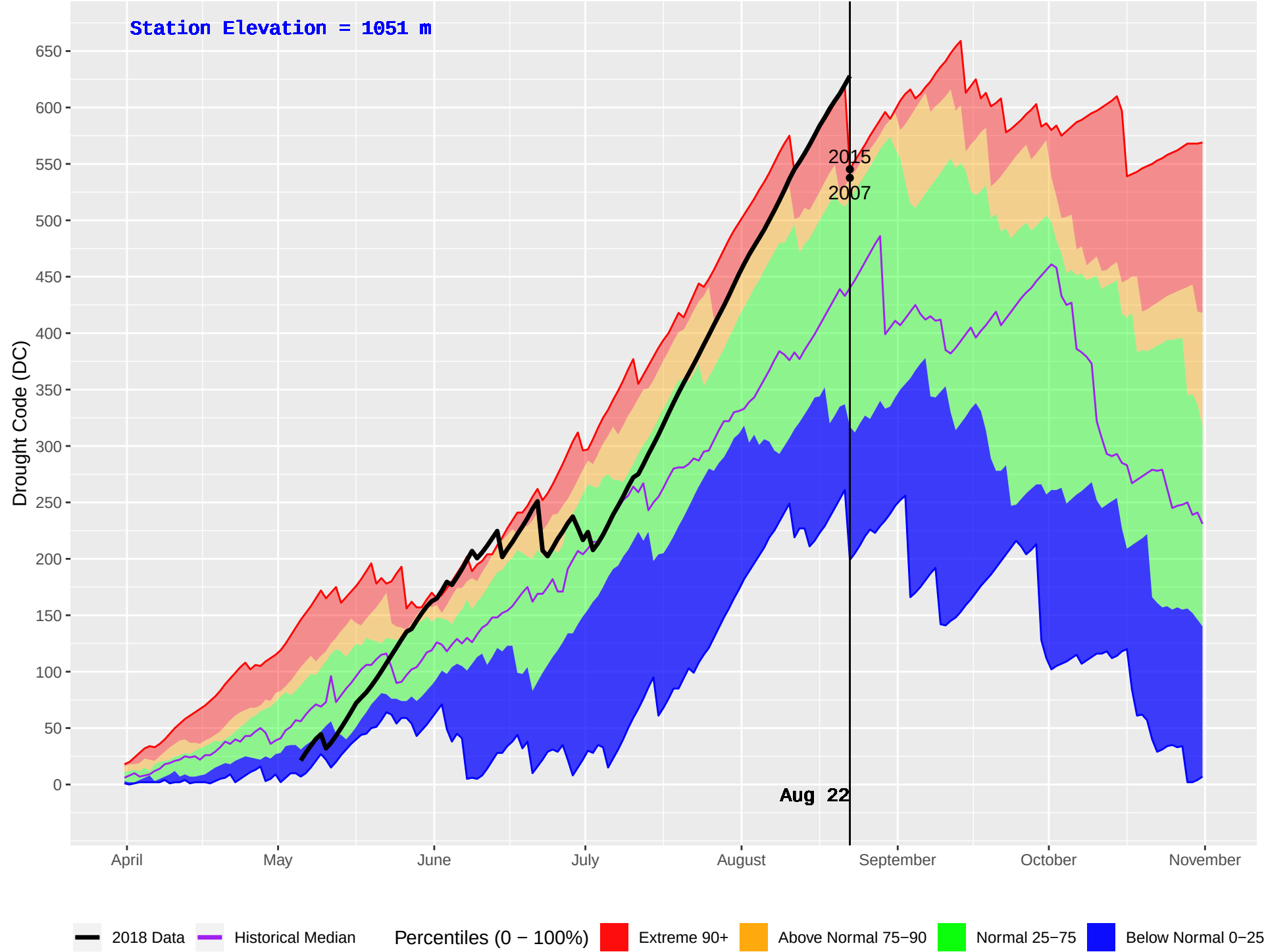
GOATHAVEN (886) : Historical (2005–2016) and Current (2018) Daily Drought Code (DC)
