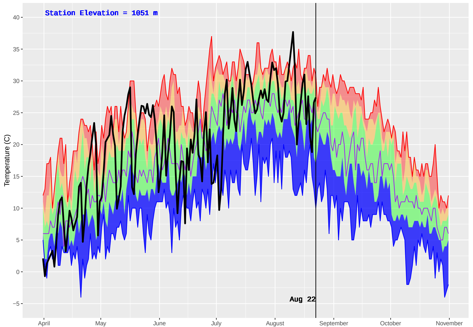
GOATHAVEN (886) : Historical (2005–2016) and Current (2018) Daily Temperature
