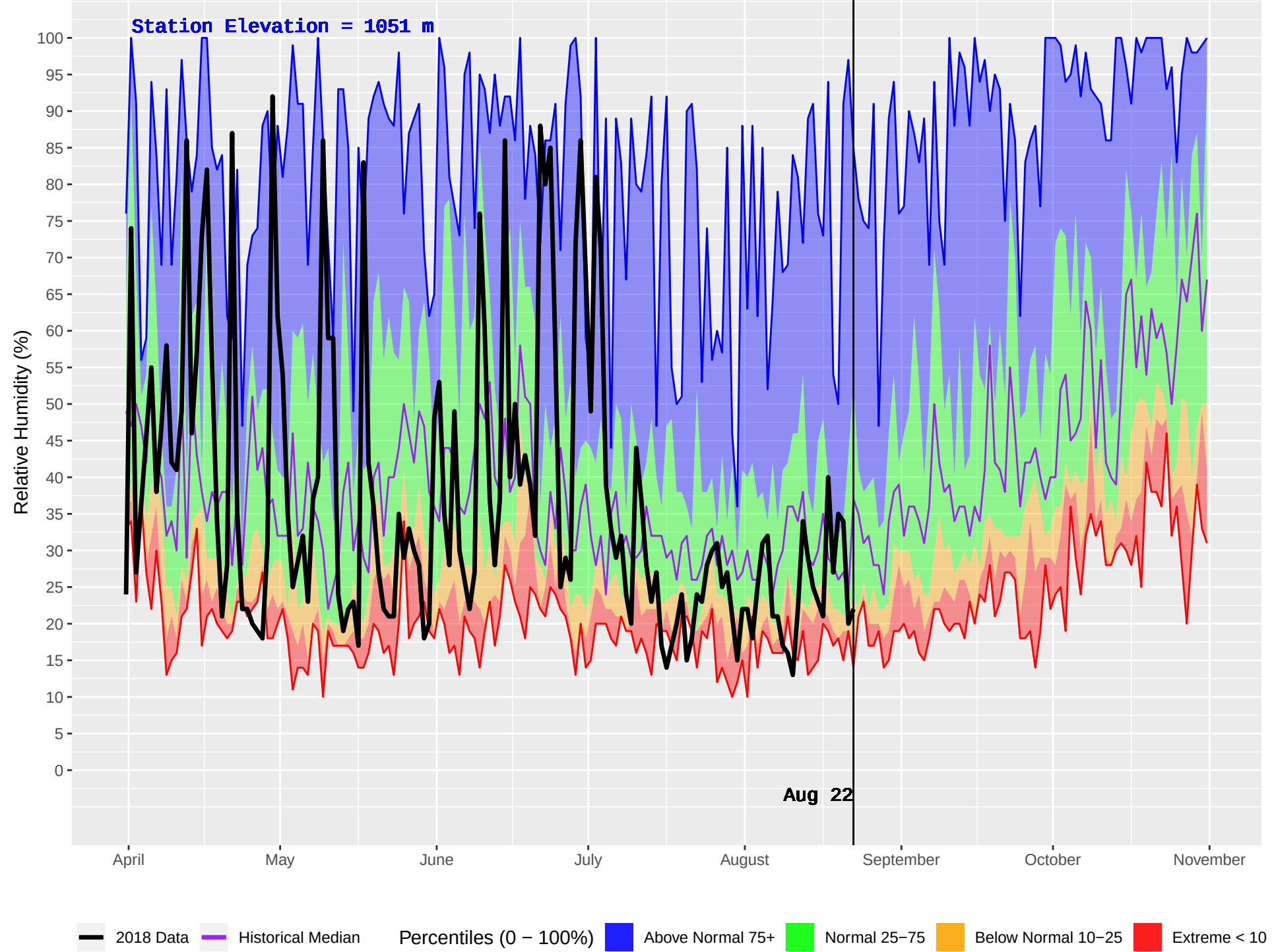
GOATHAVEN (886) : Historical (2005–2016) and Current (2018) Daily Relative Humidity
