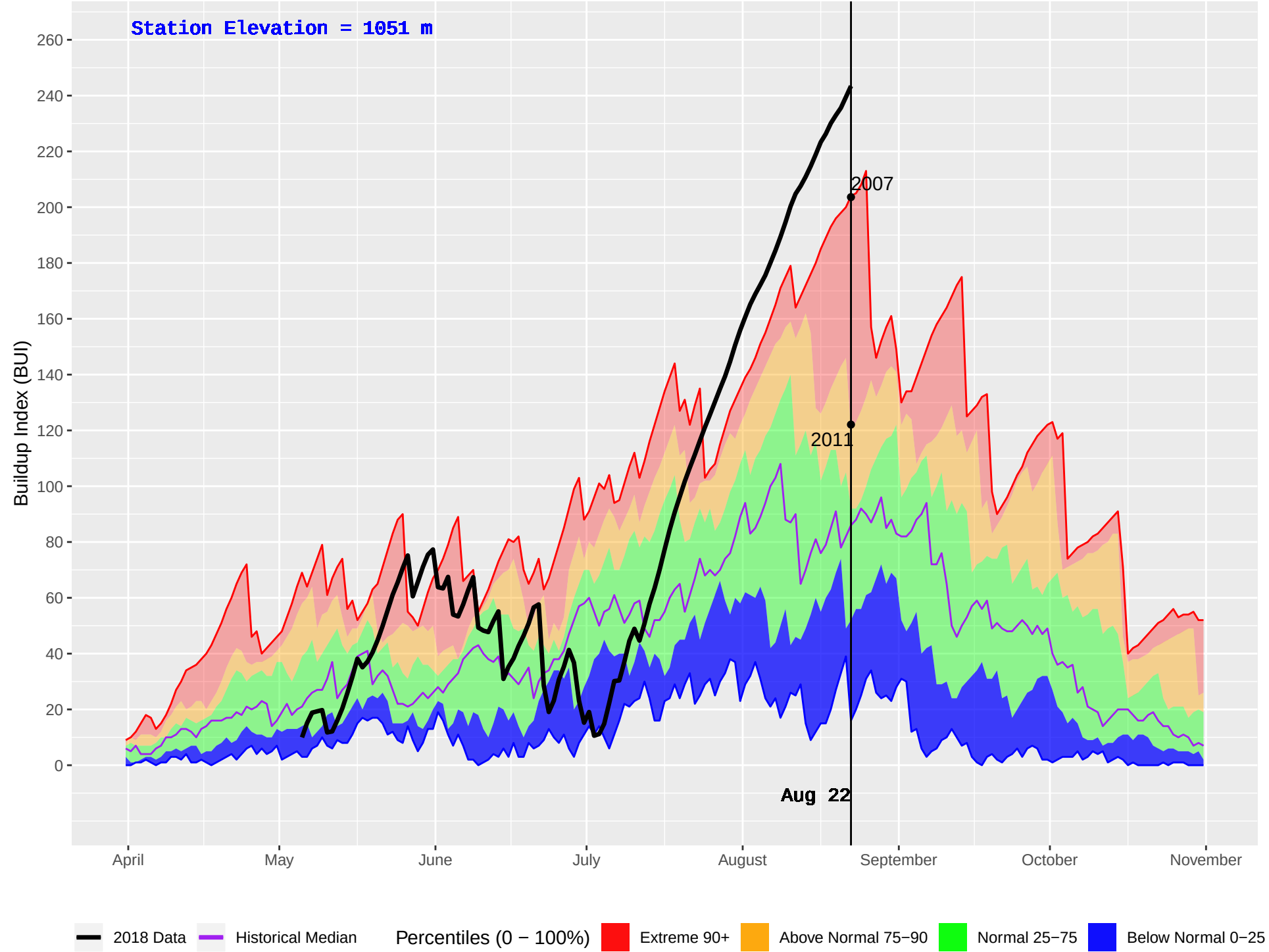
GOATHAVEN (886) : Historical (2005–2016) and Current (2018) Daily Buildup Index (BUI)
